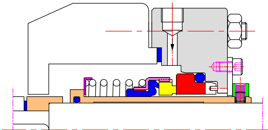
70 SERIES RUBBER BELLOW SINGLE SPRING MECHANICAL SEAL TYPE 7131 CARTRIDGE ARRANGEMENT WITH DIFFERENT API PLAN 11
